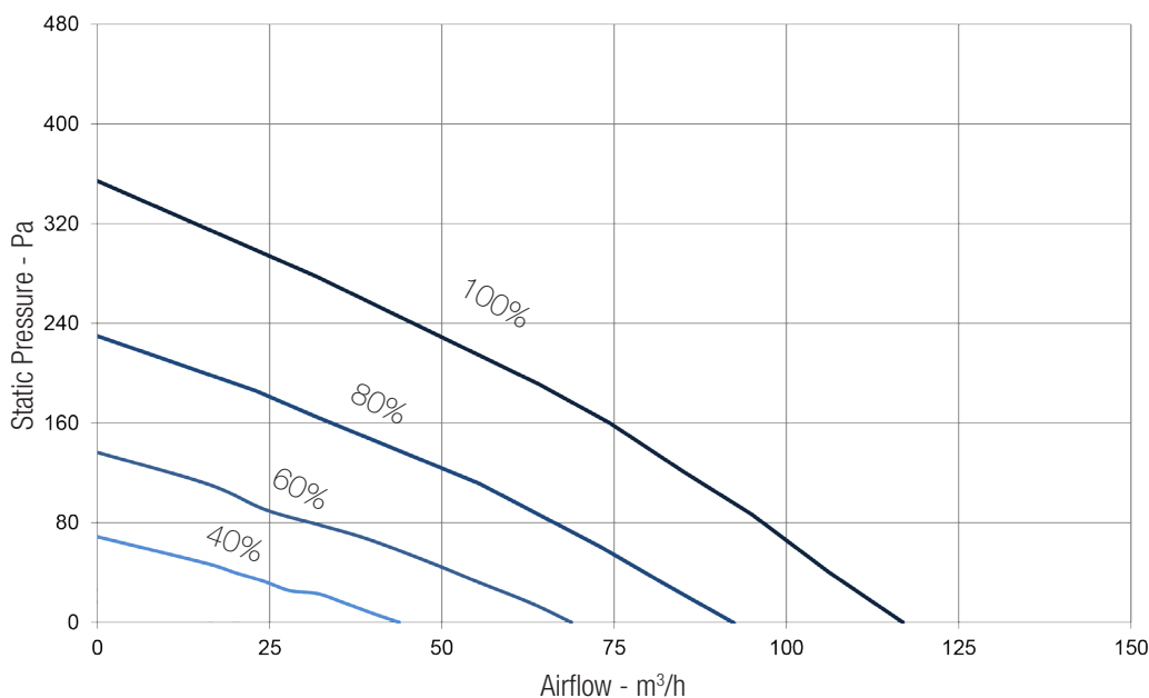
Fig. 6.b Intake curve according to Reg. 1253/2014 (ErP).
