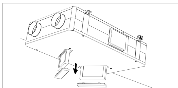
Fig. 8.f Remove the filter cap by means of the supplied bracket.
