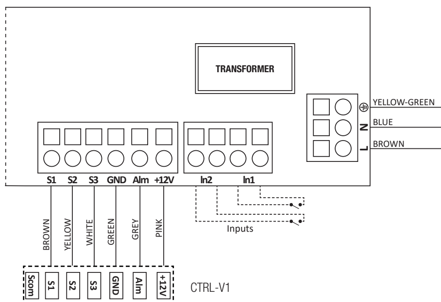
Fig. 5.k Electrical connections on the motherboard fitted in the terminal box.
