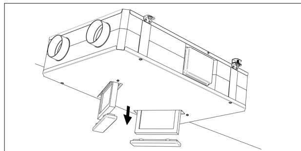
Fig. 8.c Remove the filter cap by means of the supplied bracket.
